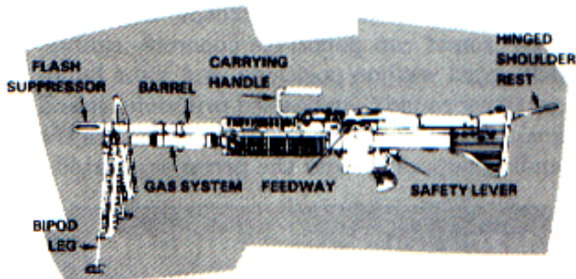
BIPOD MOUNTED
